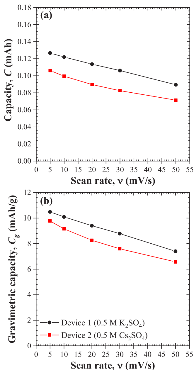
Fig. 3. (a) Capacity C(\nu) and (b) gravimetric capacity C_g(\nu) per unit mass of both electrodes as functions of scan rate \nu for Device 1 with 0.5 M K_2SO_4 and Device 2 with 0.5 M Cs_2SO_4 aqueous electrolytes.
