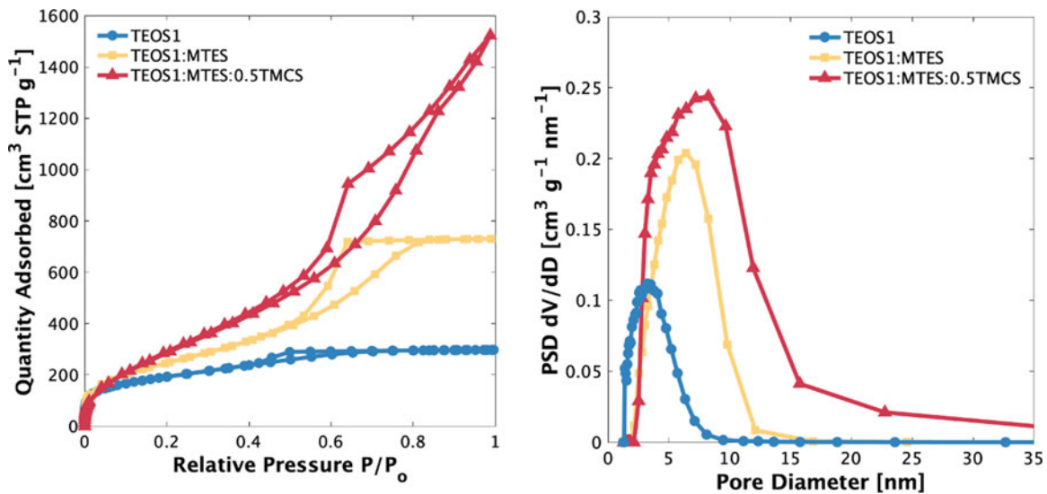
Figure 2. (a) N_2 adsorption–desorption isotherms measured at -196^\circ\text{C} , highlighting the increasing quantity adsorbed at increasing relative pressures from TEOS1 to TEOS1:MTES to TEOS1:MTES:0.5TMCS silica ambigel samples. This behavior suggests an increasing pore size and vol% porosity with increasing methyl content in the three ambigels. This trend can also be observed in the corresponding pore size distributions (b) showing an increase in average pore size and width of pore size distribution with increasing methyl content (see Tables 1 and 2).
