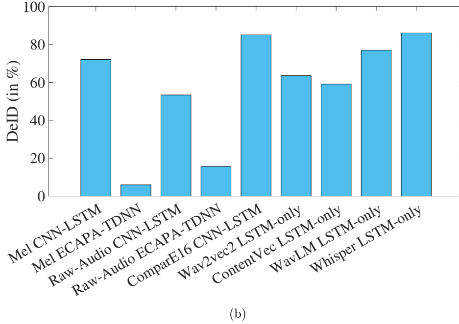
Figure 6.4: (a) G_{VD} in dB and (b) De - ID in %, respectively, for each experiment when speaker disentanglement is applied in the form of LECE. The X-axis of each plot represents the 9 different feature-model combinations.
