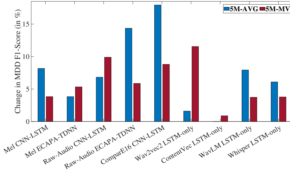
Figure 6.1: Relative improvements, in percentage, in MDD classification F1-Score when speaker disentanglement is applied in the form of LEV. The X-axis of each plot represents the 9 different feature-model combinations. 5M-AVG and 5M-MV refer to the averaging and majority voting aggregation of the 5 models, respectively. A higher value indicates a greater improvement in depression detection after speaker disentanglement is applied.
