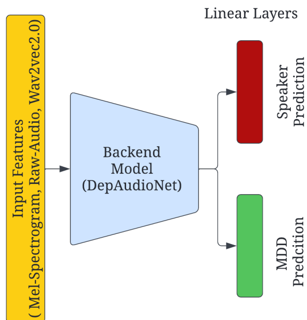
Figure 5.1: Block diagram representing adversarial disentanglement of speaker and depression characteristics.
