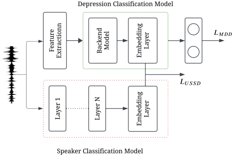
Figure 7.1: The unsupervised speaker disentanglement method (USSD) aims to minimize cosine similarity between latent spaces of depression classification and speaker classification models.
