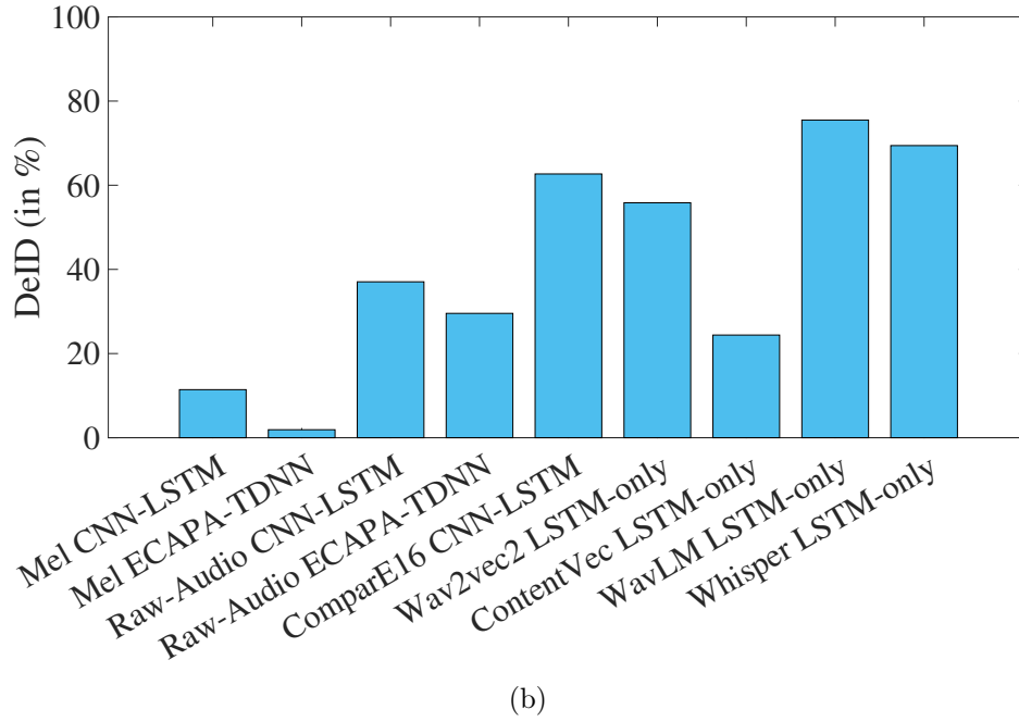
Figure 6.6: (a) G_{VD} in dB and (b) De-ID in %, respectively, for each experiment when speaker disentanglement is applied in the form of LEKLD. The X-axis of each plot represents the 9 different feature-model combinations.
