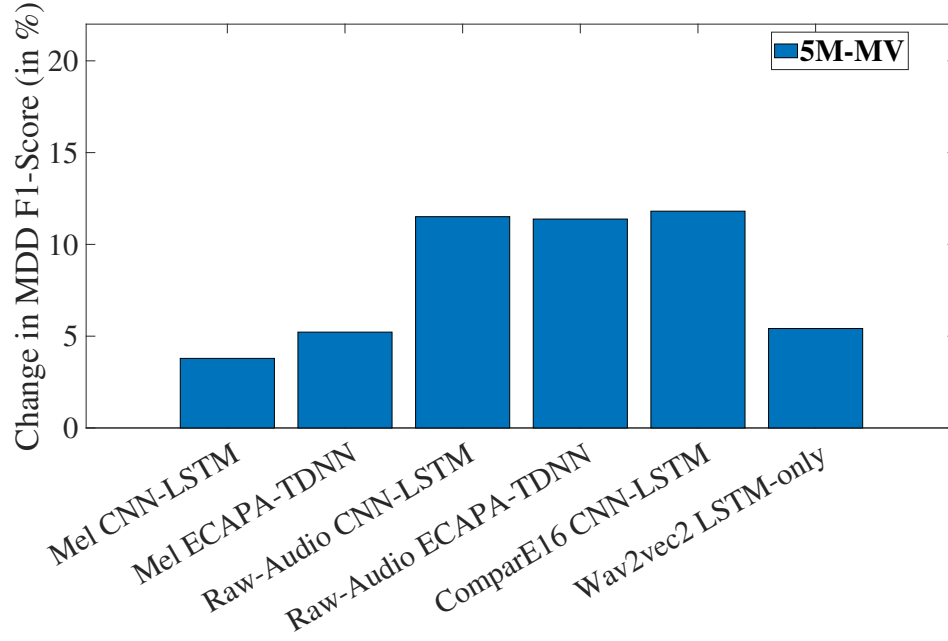
Figure 7.2: Relative improvements, in percentage, in MDD classification F1-Score when speaker disentanglement is applied in the form of USSD. The X-axis of each plot represents the 6 different feature-model combinations. 5M-MV refer to the averaging and majority voting aggregation of the 5 models, respectively. A higher value indicates a greater improvement in depression detection after speaker disentanglement is applied.
