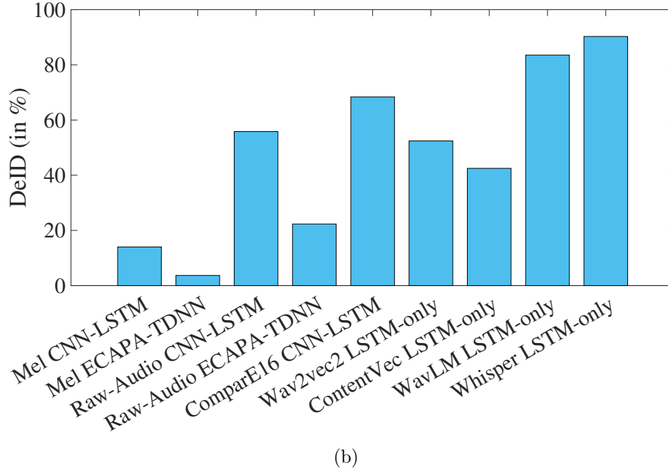
Figure 5.3: (a) G_{VD} in dB and (b) De - ID in %, respectively, for each experiment when speaker disentanglement is applied in the form of ADV. The X-axis of each plot represents the 9 different feature-model combinations.
