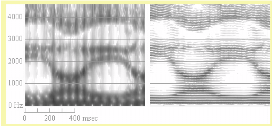
Figure 4.1: Wide-band and Narrow-band spectrograms for the same speech signal
