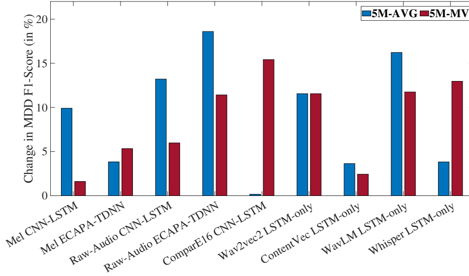
Figure 6.3: Relative improvements, in percentage, in MDD classification F1-Score when speaker disentanglement is applied in the form of LECE. The X-axis of each plot represents the 9 different feature-model combinations. 5M-AVG and 5M-MV refer to the averaging and majority voting aggregation of the 5 models, respectively. A higher value indicates a greater improvement in depression detection after speaker disentanglement is applied.
