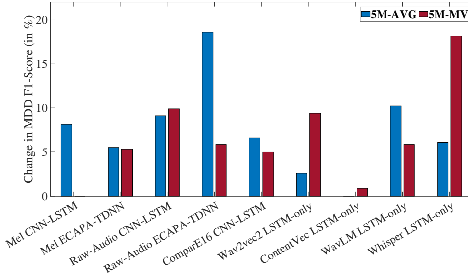
Figure 6.5: Relative improvements, in percentage, in MDD classification F1-Score when speaker disentanglement is applied in the form of LEKLD. The X-axis of each plot represents the 9 different feature-model combinations. 5M-AVG and 5M-MV refer to the averaging and majority voting aggregation of the 5 models, respectively. A higher value indicates a greater improvement in depression detection after speaker disentanglement is applied.
