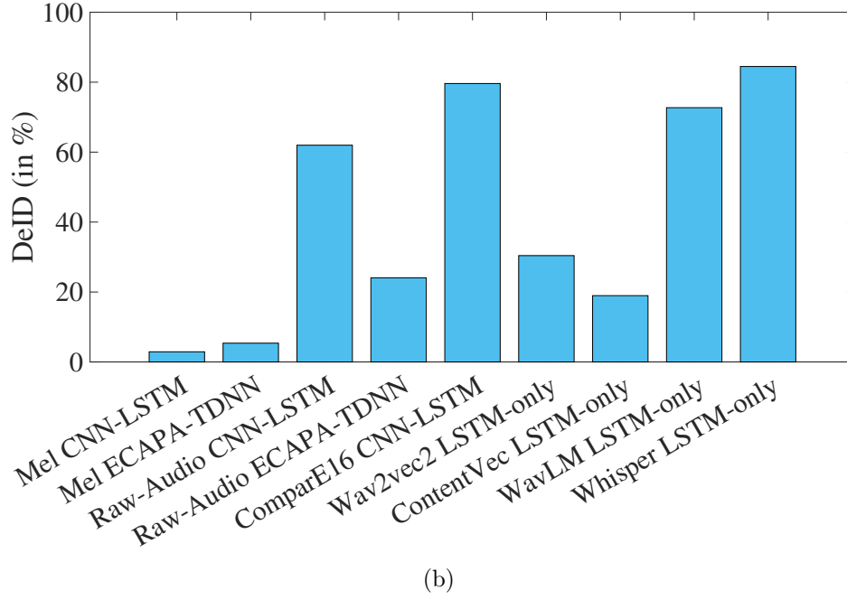
Figure 6.2: (a) G_{VD} in dB and (b) De - ID in %, respectively, for each experiment when speaker disentanglement is applied in the form of LEV. The X-axis of each plot represents the 9 different feature-model combinations.
