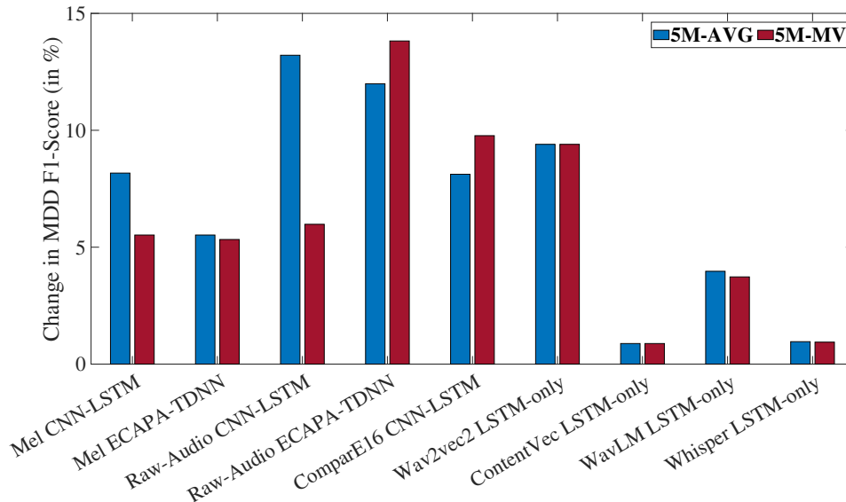
Figure 5.2: Relative improvements, in percentage, in MDD classification F1-Score when speaker disentanglement is applied in the form of ADV. The X-axis of each plot represents the 9 different feature-model combinations. 5M-AVG and 5M-MV refer to the averaging and majority voting aggregation of the 5 models, respectively. A higher value indicates a greater improvement in depression detection after speaker disentanglement is applied.
