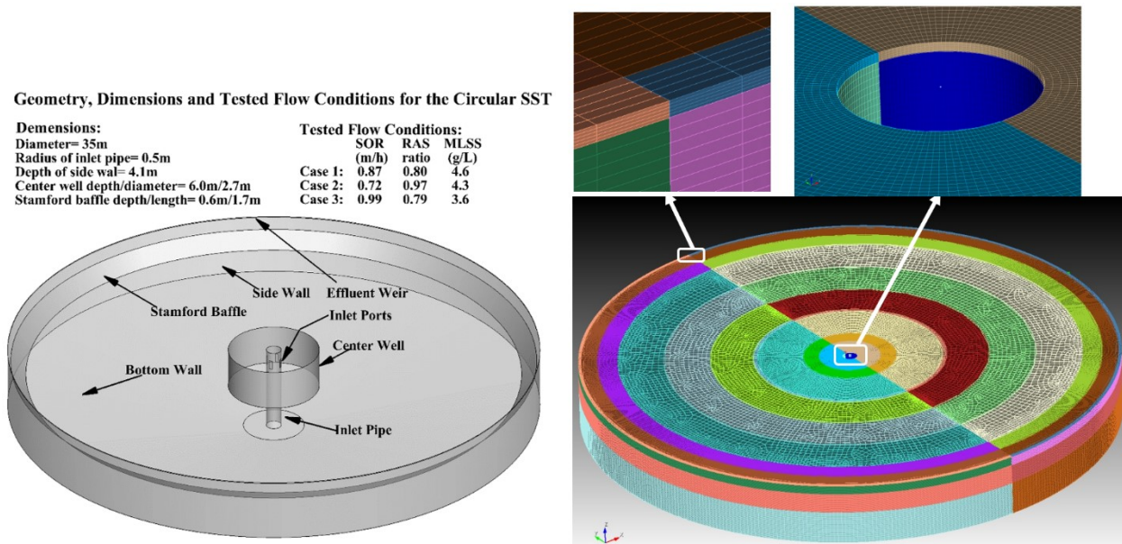
Figure 9-1. Geometry, dimensions, the tested flow conditions (left) and mesh (right) for the circular SST
