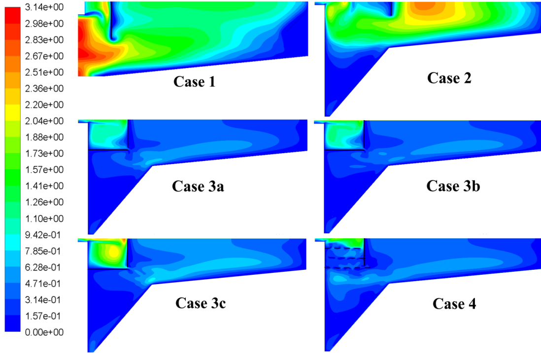
Figure 5-5. Predictions of the turbulent viscosity (kg/m-s) by the buoyancy-decoupled SKE models for the circular SSTs (Cases 1 to 4, respectively).
