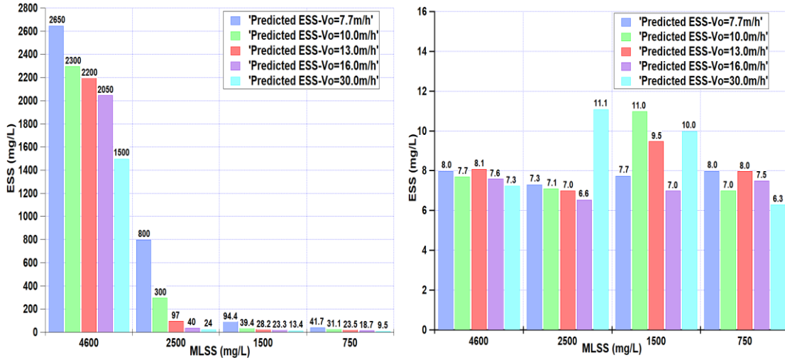
Figure 4-4. Predicted ESS with four different MLSS concentrations and five Stokes velocities V_o : (a) buoyancy-decoupled; (b) buoyancy-coupled. ( Q=1500 \text{ m}^3/\text{h} , RAS=0.8 ).
