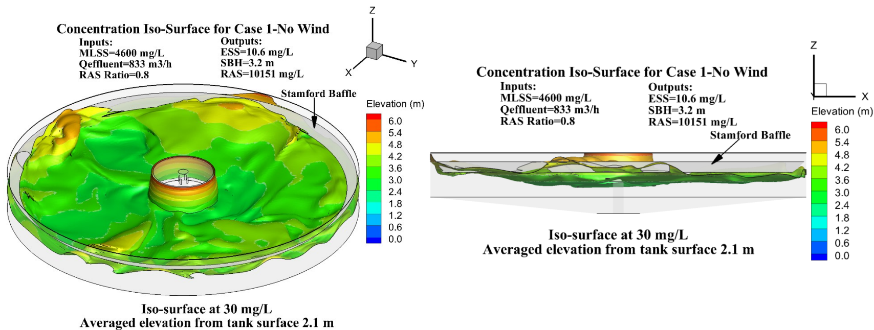
Figure 9-5. Concentration iso-surface at 30 mg/L under the calm condition for the Case 1. Note the four inlet ports in the very center of the SST.
