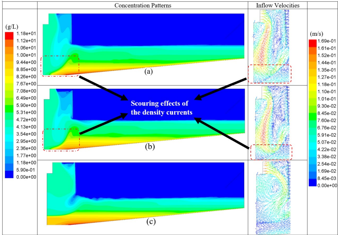
Figure 3-8. Flow and concentration contours for the Test 1 of Darvill SST predicted by (a) SKE, (b) RNG k-\epsilon and (c) Realizable k-\epsilon turbulence models.
