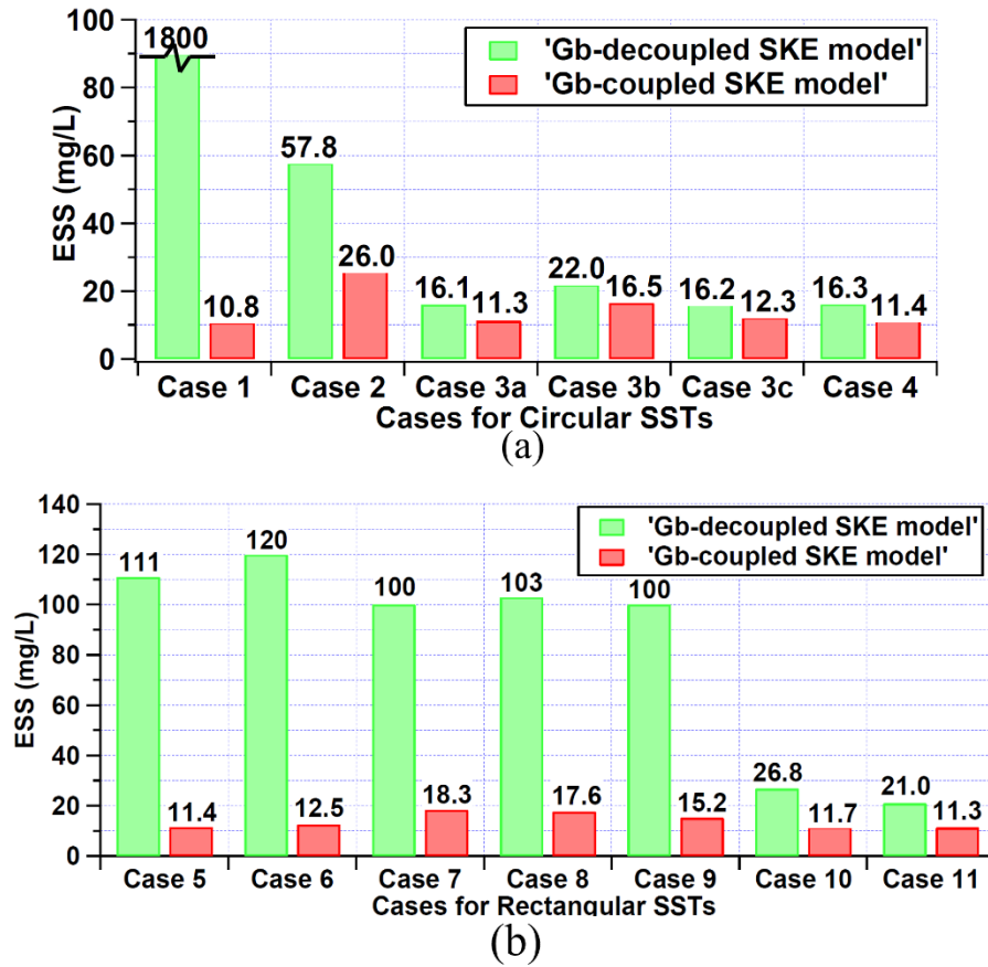
Figure 5-4. Predictions of the ESS by the G_b -decoupled/coupled turbulence models with these 13 cases (a: circular SSTs; b: rectangular SSTs)
