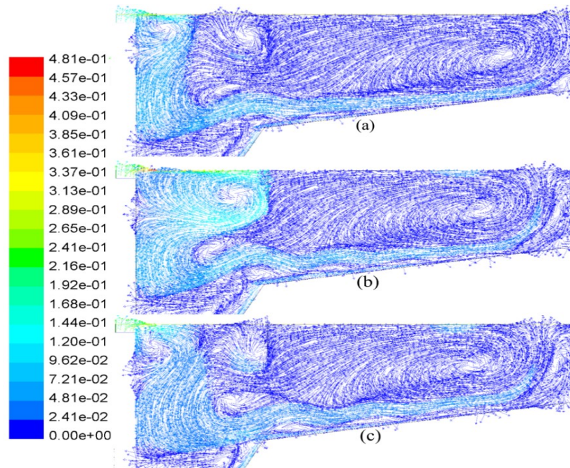
Figure 3-12. Comparison of the predicted flow contours (m/s) for the Witney SST under the maximum hydraulic loading condition: (a) SKE model, (b) RNG model, (c) Realizable k\text{-}\varepsilon model.
