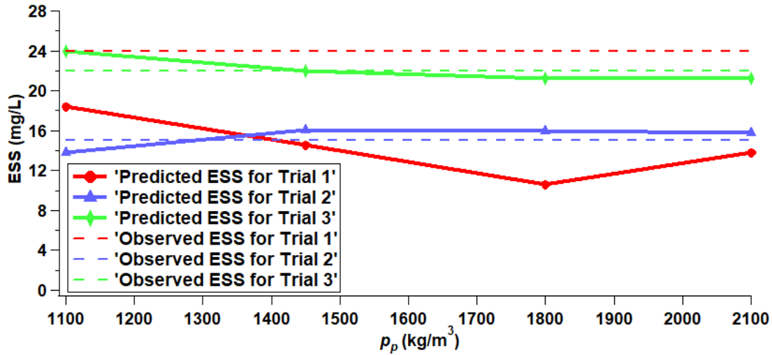
Figure 6-7. Prediction of ESS (mg/L) respect to \rho_p ( \text{kg/m}^3 ) for Trials 1 to 3.
