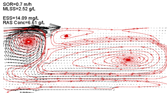
Figure 7-16. streamline after geometry modification (simulation 16)
