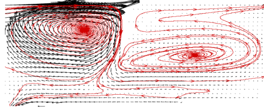
Figure 7-11. Streamline for simulation 3
