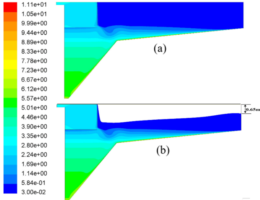
Figure 6-6. Predictions of sludge concentration profiles (g/L) for the Trail 3 (a (top): r_p=3.86 L/g; b (bottom): r_p=30.00 L/g). Only the regions with sludge concentration higher than 30 mg/L are shown.
