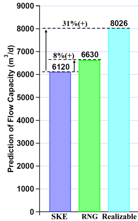
Figure 3-11. Prediction of the flow capacity by the SKE, RNG and Realizable k\text{-}\varepsilon turbulence models.
