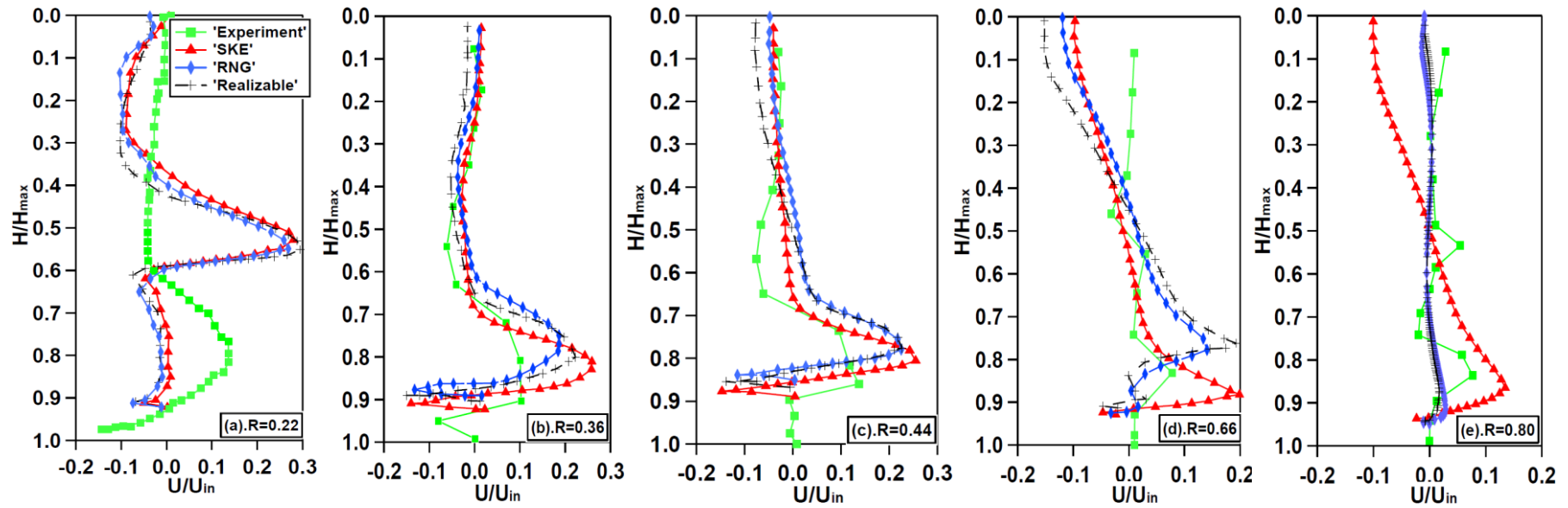
Figure 3-4. Comparison of radial velocity profiles by various turbulence models with field measurements for Witney SST. R is the ratio between the radial distance of the vertical measurement location to the radius of tank.
