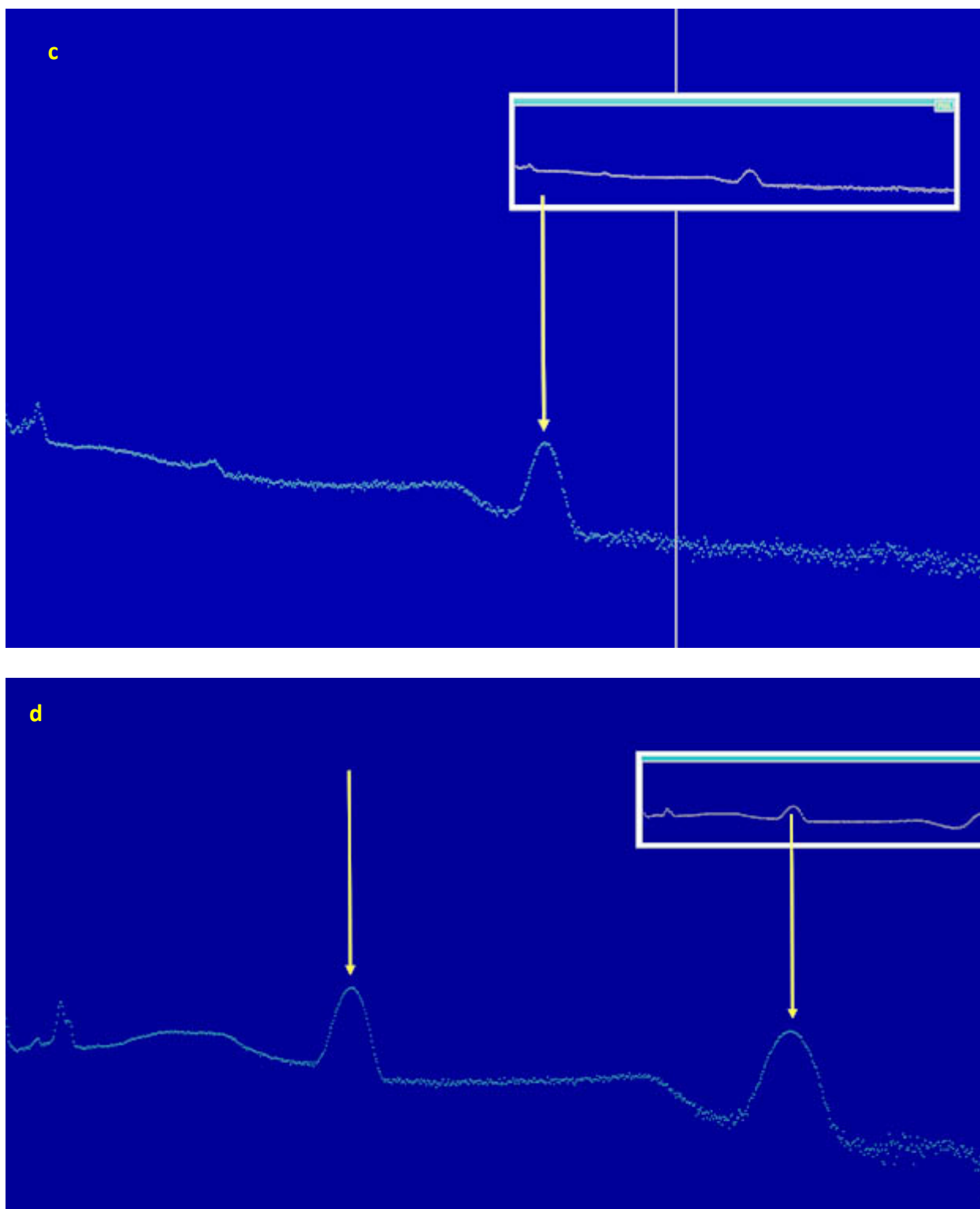
Figure 4.5-a to d: ten minutes counting of the a: ^{60}\text{Co} , b: ^{137}\text{Cs} , c: ^{40}\text{K} and d: ^{22}\text{Na} standards
