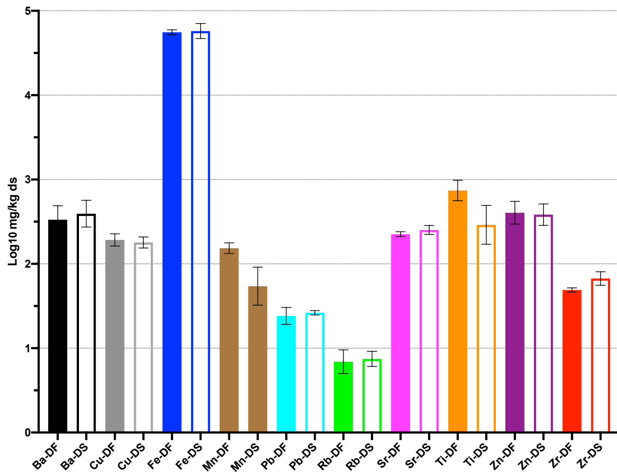
Figure 4-5. Average heavy metal contents in log 10 mg/kg ds in digester feed (DF) and digested sludge (DS) at AD4.
