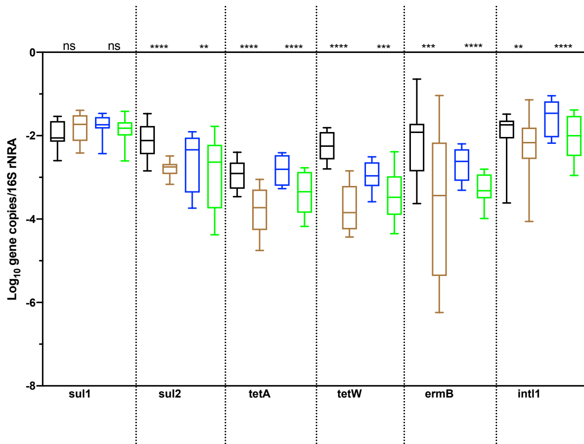
Figure 2-8. Relative gene abundance of the target ARGs per 16S rRNA, in the three long SRT plants influent (black) and effluent (brown) samples and the three short SRT plants influent (dark blue) and effluent (green). Different genes are separated by vertical lines. The results are expressed in log 10 copies per 16S rRNA. The boxes represent the 1st and 3rd quartiles. The middle line represents the median, and the whiskers represent the min and max values. Significant differences in gene presence after treatment were assessed by a paired t test and values are indicated above each gene: p > 0.05 (ns), p < 0.05 (*), p < 0.01 (**), p < 0.001 (***), and p < 0.0001 (****).
