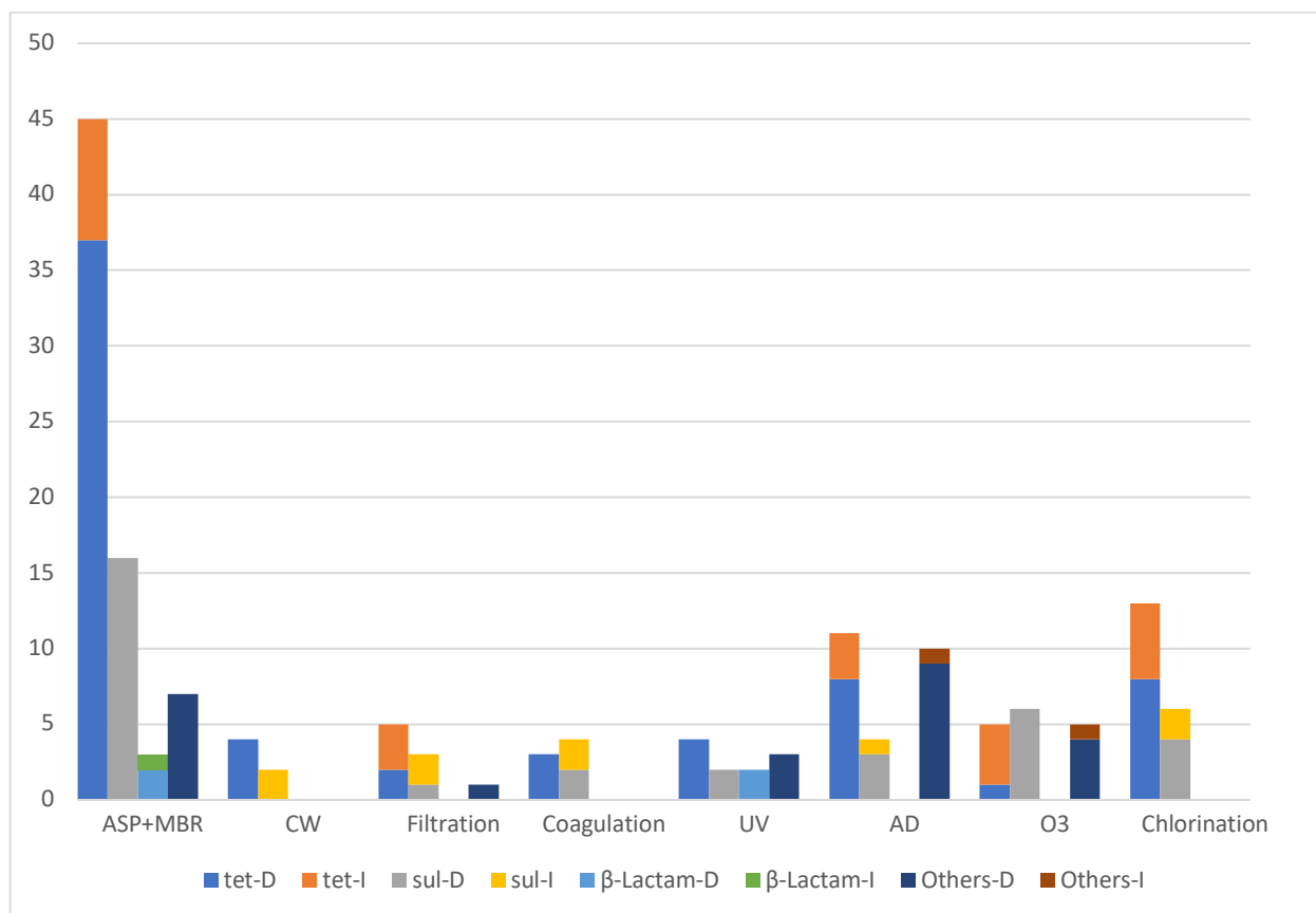
Figure 1-2. Comparison of tetracycline ( tet ), sulfonamide ( sul ), \beta -Lactam and other antibiotic resistance genes that are decreased and increased in treatment processes, including activated sludge process (ASP) and membrane bio-reactor (MBR), constructed wetland (CW), filtration, UV disinfection, anaerobic digester (AD), ozonation (O 3 ), and chlorination. (Note: D indicates decrease and I indicates increase. For example, tet-D indicates numbers of decreased observations for tetracycline resistance genes and tet-I indicates numbers of increased observations for tetracycline resistance genes.)
