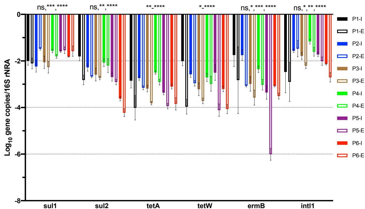
Figure 2-7. Relative gene abundance of target ARGs at each plant's influent and effluent. The results are expressed in log10 copies per 16S rRNA. Significance differences of each plant were assessed by a paired t test and values are indicated above each gene: p > 0.05 (ns), p < 0.05 (*), p < 0.01 (**), p < 0.001 (***), and p < 0.0001 (****).
