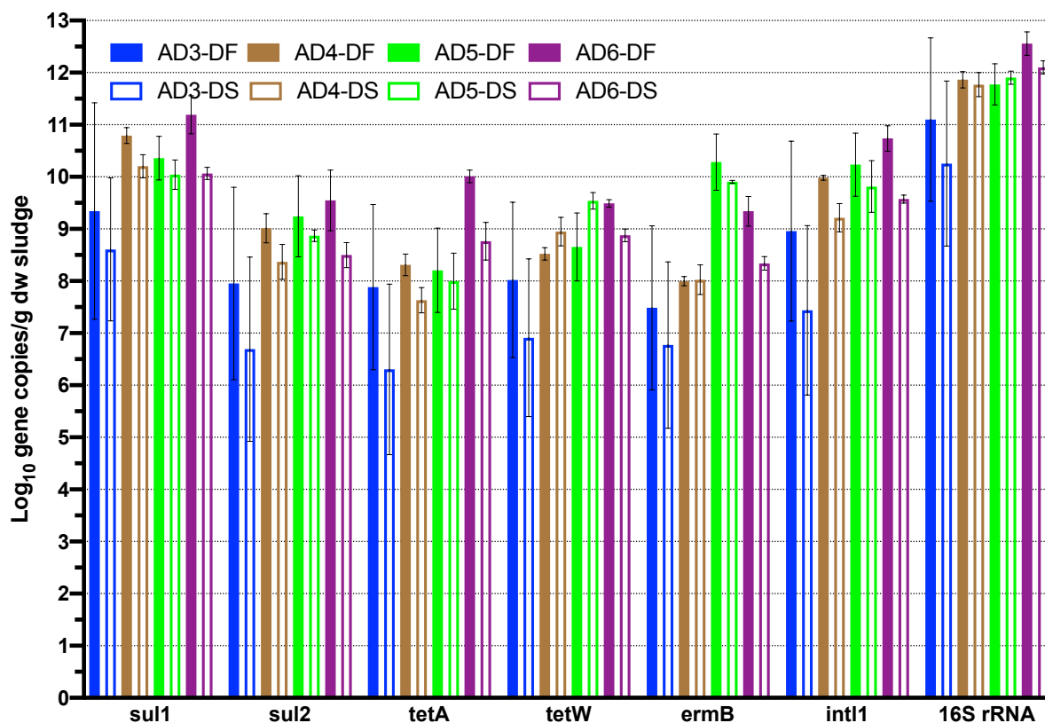
Figure 3-2. Absolute gene abundance of each target ARG at each of the four plants' anaerobic digester. The results are expressed in \log_{10} copies per g dw sludge.
