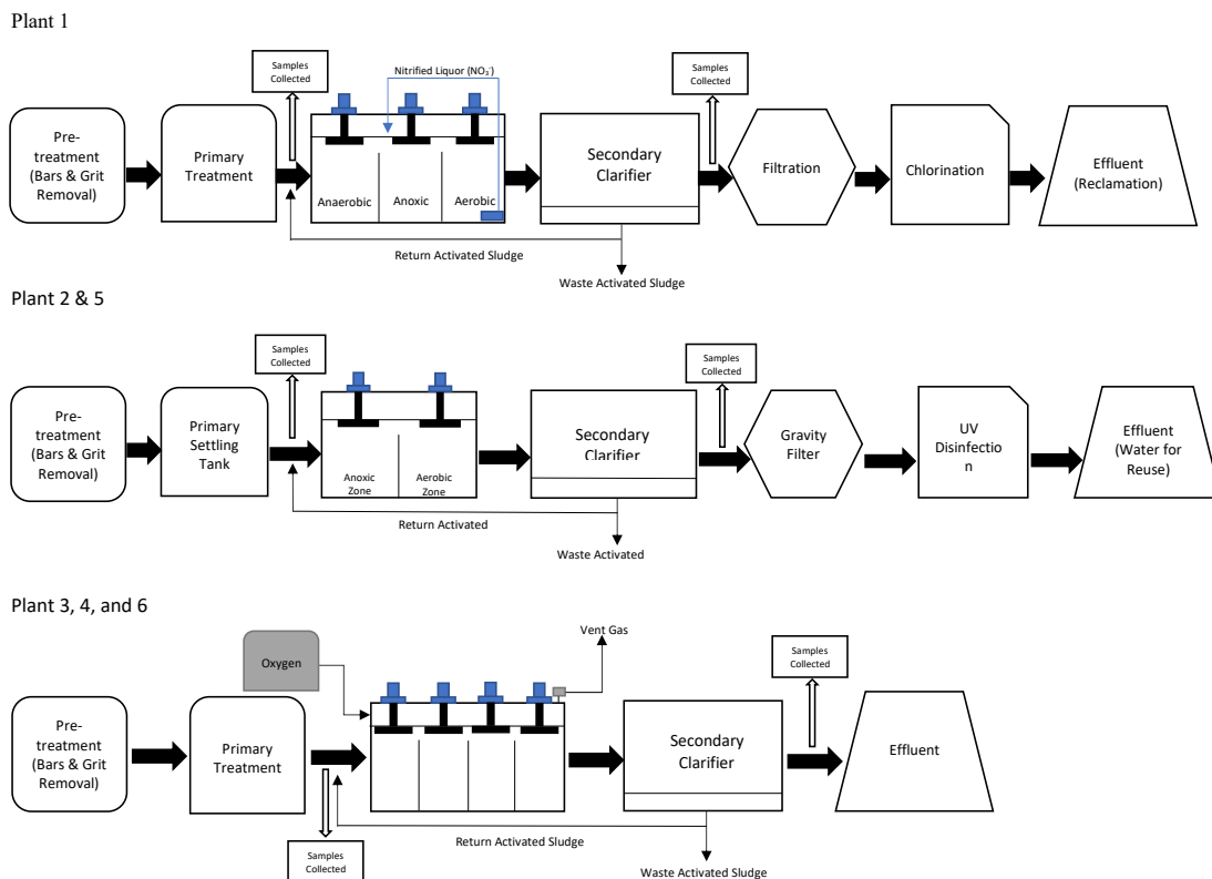
Figure 2-1. Schematic layout of the six wastewater treatment plants with activated sludge processes.
