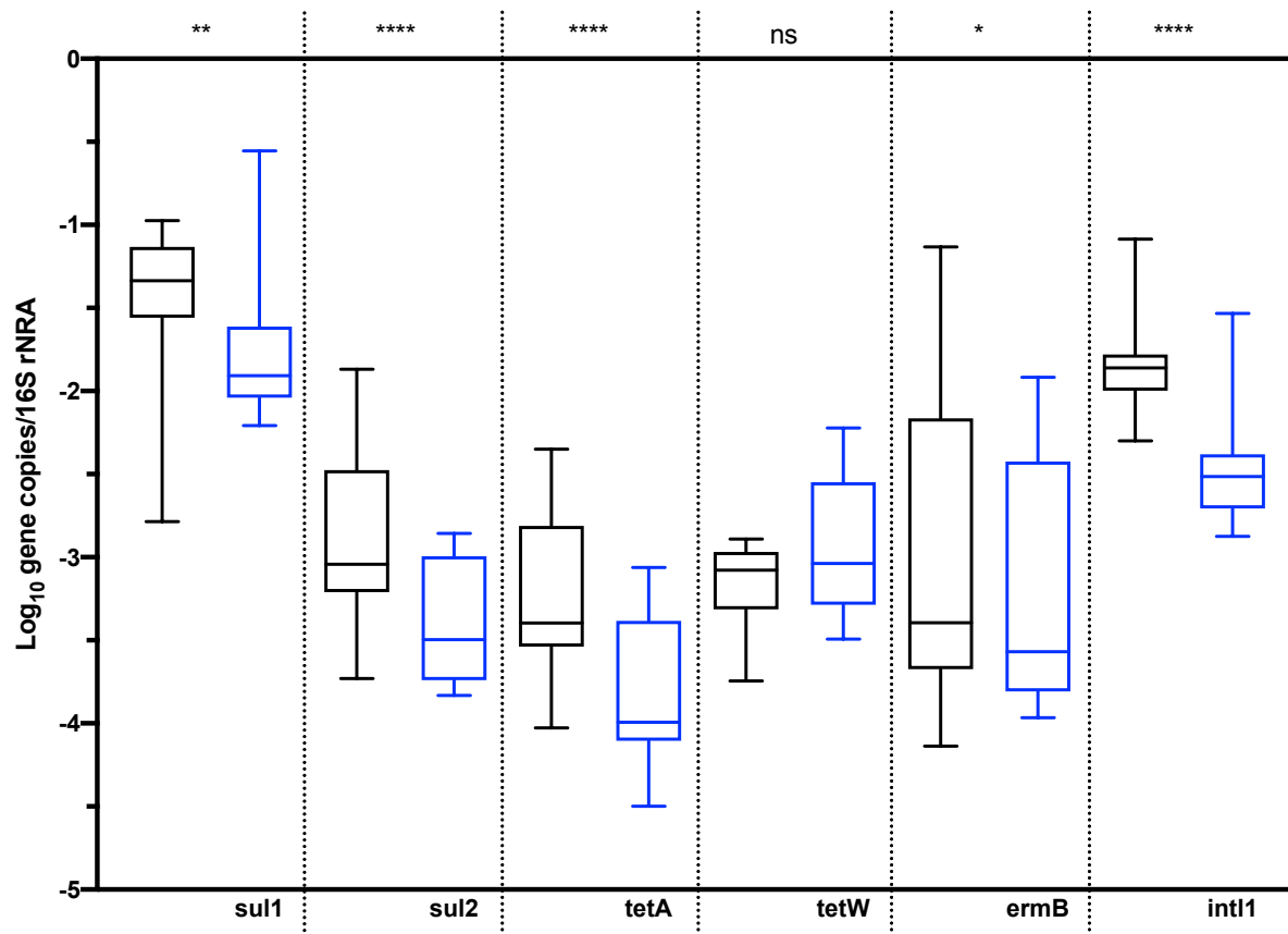
Figure 3-8. Relative gene abundance of the target ARGs, in the four anaerobic digesters' digester feed (black) and digested sludge (blue) samples. Different genes are separated by vertical lines. The results are expressed in log 10 copies per 16S rRNA. The boxes represent the 1st and 3rd quartiles. The middle line represents the median, and the whiskers represent the min and max values. Significant differences in gene presence after treatment were assessed by a paired t test and values are indicated above each gene: p > 0.05 (ns), p < 0.05 (*), p < 0.01 (**), p < 0.001 (***), and p < 0.0001 (****).
