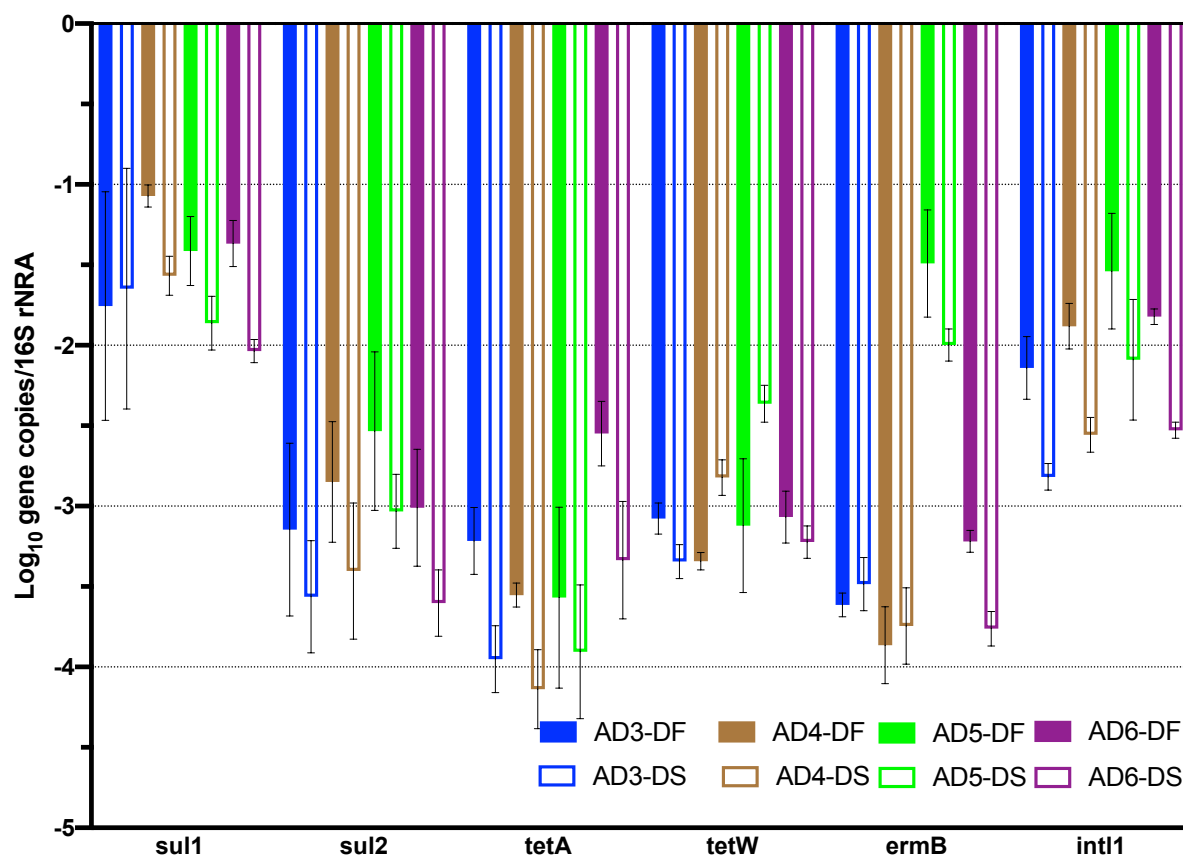
Figure 3-6. Relative gene abundance of each target ARG at each of the four plants' anaerobic digester. The results are expressed in log 10 copies per 16S rRNA.
