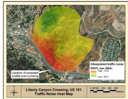
Figure 4-7: Sound Intensity at the Proposed Overcrossing
