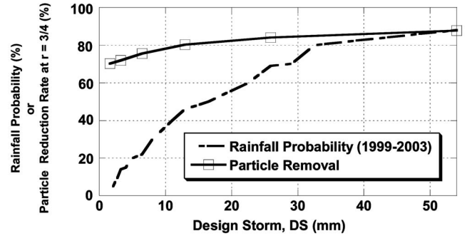
Fig. 9. Optimized particle reduction rate and rainfall probability with respect to design storm (rainfall probability means the probability of an event rainfall to be less than a stated design storm)
