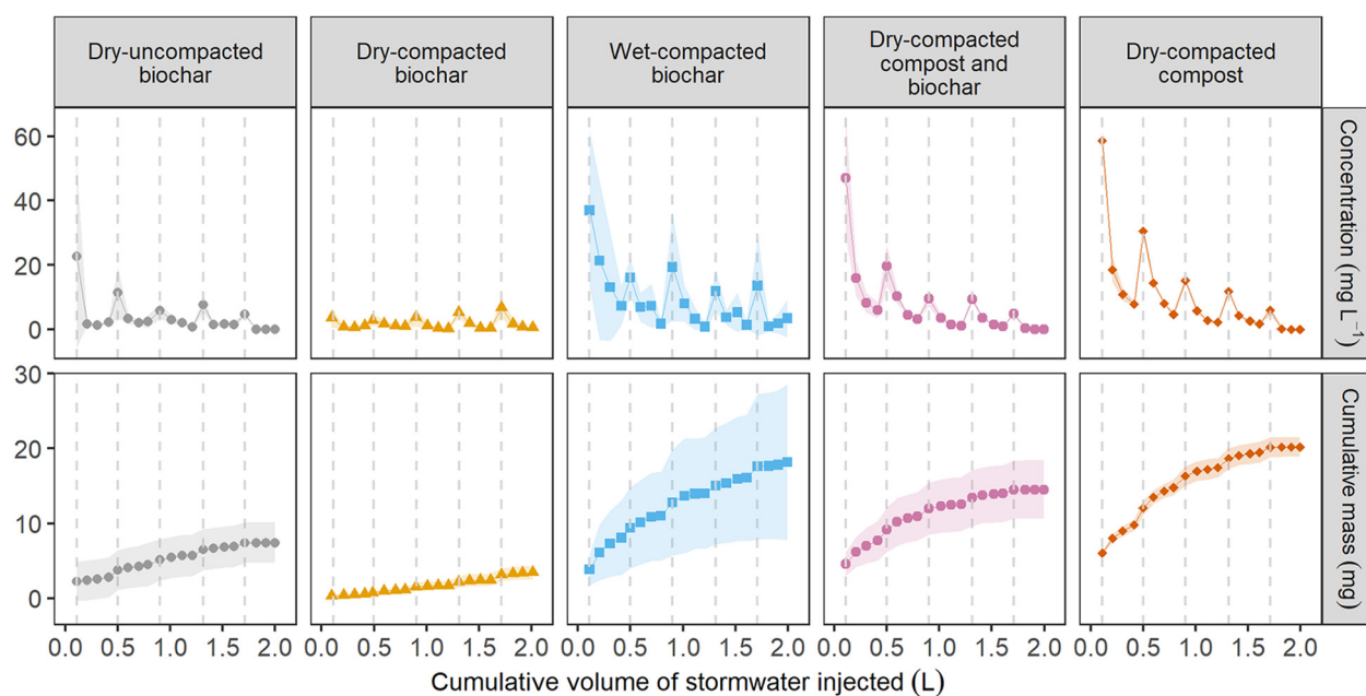
Fig. 3. Concentration (top) and cumulative mass (bottom) of particles released from biofilters packed with biochar or compost under different compaction conditions. Dashed lines indicate the start of rainfall infiltration events. Shaded area indicates one standard deviation over mean value from triplicate columns.
