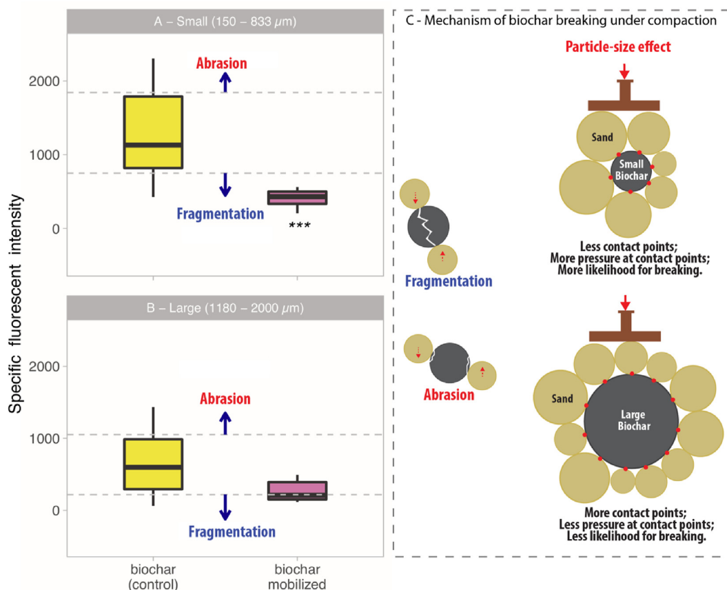
Fig. 5. Specific fluorescent intensity of packed biochar and mobilized biochar for (A) small biochar column and (B) large biochar column. *** indicates a p-value < 0.001. (C) The illustration shows the difference in breakage mechanisms (abrasion vs. fragmentation or splitting) and dissipation of compaction energy based on biochar size.
