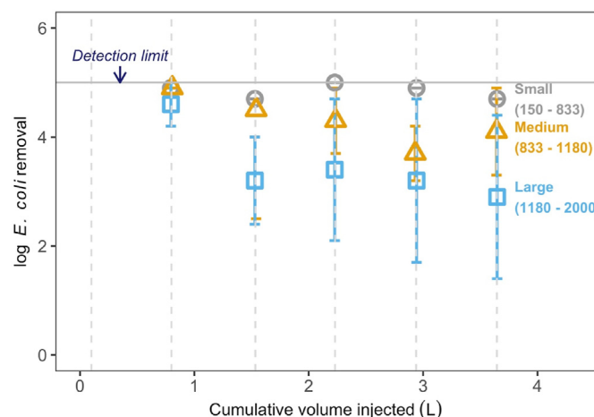
Fig. 3. Removal of E. coli during rainfall events. The error bars indicate one standard deviation over mean from triplicate columns with duplicate measurements per column ( n = 6 ). The vertical dashed lines indicate the start of a rainfall event.
