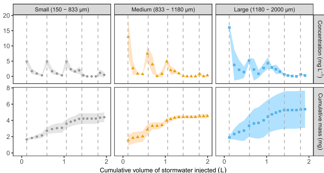
Fig. 1. Release of particles from compacted biochar-sand biofilters during intermittent infiltration of stormwater. Points represent mean value obtained from triplicated columns, and the shaded area represents one standard deviation over the mean.
