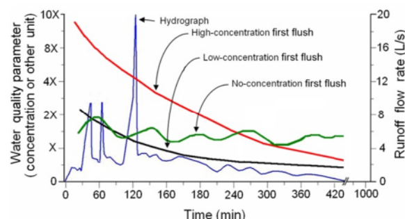
Fig. 2. A definition sketch of concentration first flush
