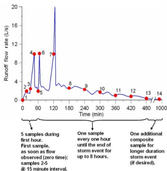
Fig. 1. Sampling strategy to evaluate first flush characterization
