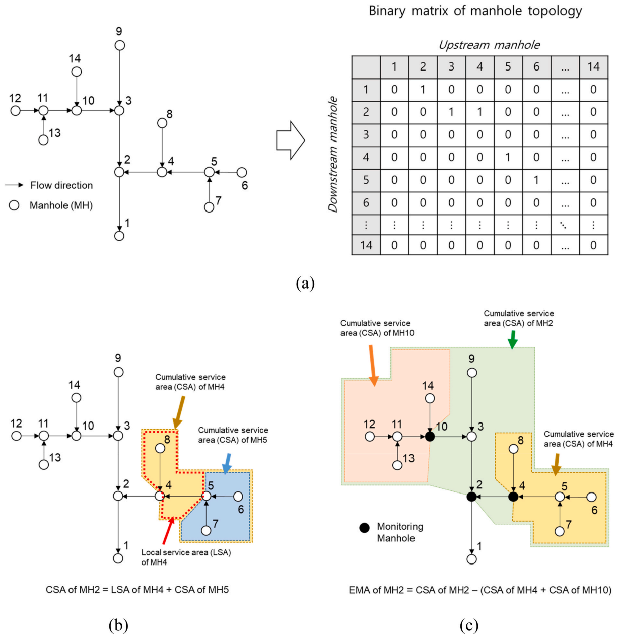
Fig. 1. Concepts of manhole topology database, the cumulative service area, and the effective monitoring area for a hypothetical sewer network: (a) Construction of a binary matrix representing the manhole topology. Direct connection and no direct connection (or no connection) between two manholes are indicated by 1 and 0, respectively; (b) Illustration of the cumulative service area (CSA); (c) illustration of the effective monitoring area (EMA).
