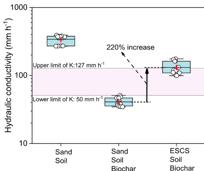
Fig. 1. Comparison of hydraulic conductivity of three soil media mixtures under compaction: sand (75% by volume) and soil (25%); sand (50%), soil (25%), and biochar (25%); ESCS (50%), soil (25%), and biochar (25%). The shaded area indicates the design hydraulic conductivity of the roadside soil. Plus (+) signs indicate the mean hydraulic conductivity of a total of 12 measurements in triplicate columns per media mixture type.
