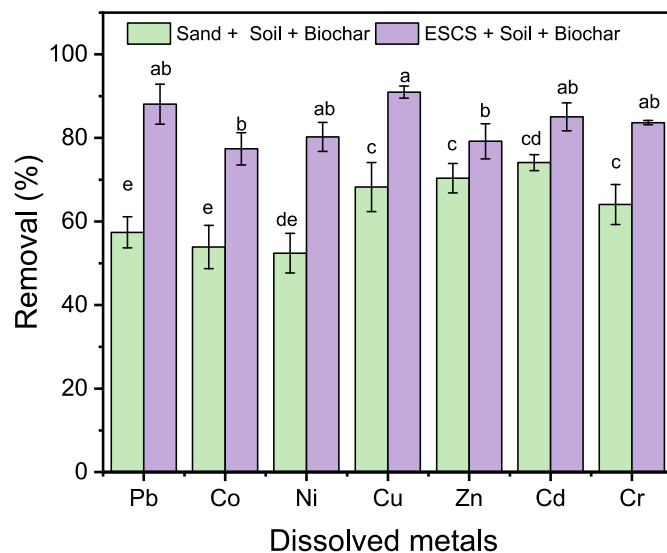
Fig. 4. The metal removal performance of ESCS amended soil media mixture after exposure of 700 PV metal contaminated natural stormwater. Error bars indicate one standard deviation over the mean based on the results from triplicate columns. Means that do not share a letter are significantly different.
