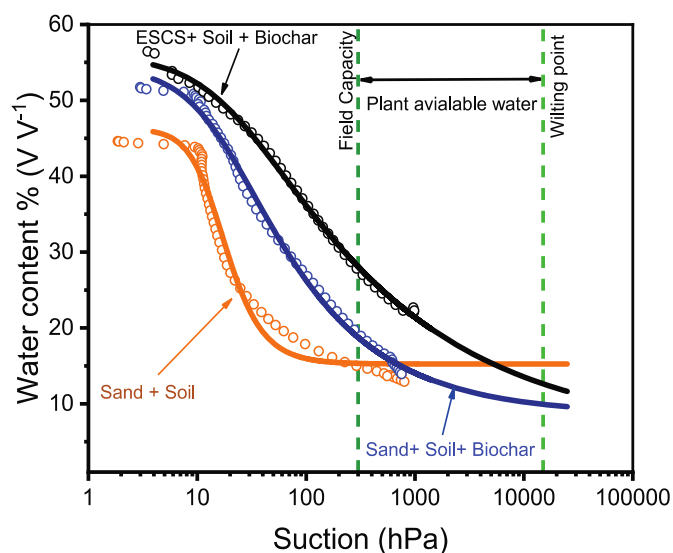
Fig. 2. Comparison of water retention behavior of three types of soil media mixtures. The solid lines indicate the van Genuchten (1980) unimodal fit for the experimental data. The plant-available water is the difference between the vertical dash lines of field capacity and the permanent wilting point.
