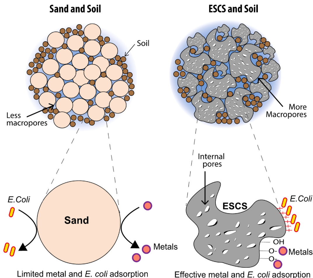
Fig. 5. Conceptual illustration showing ESCS could have many advantages over sand due to their shape, internal pores, and reactive surfaces.
