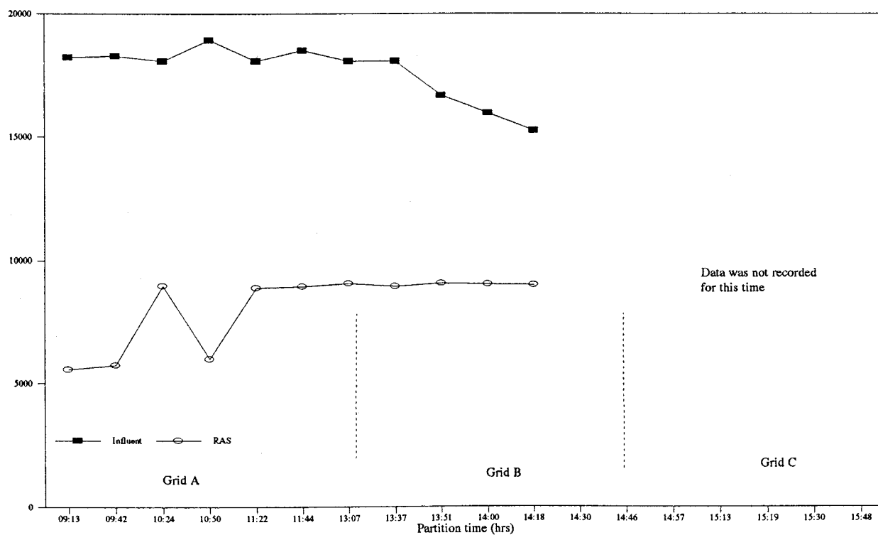
(b) Influent and RAS flow rate
