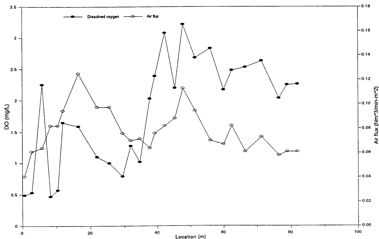
(b) Dissolved oxygen and air flux
