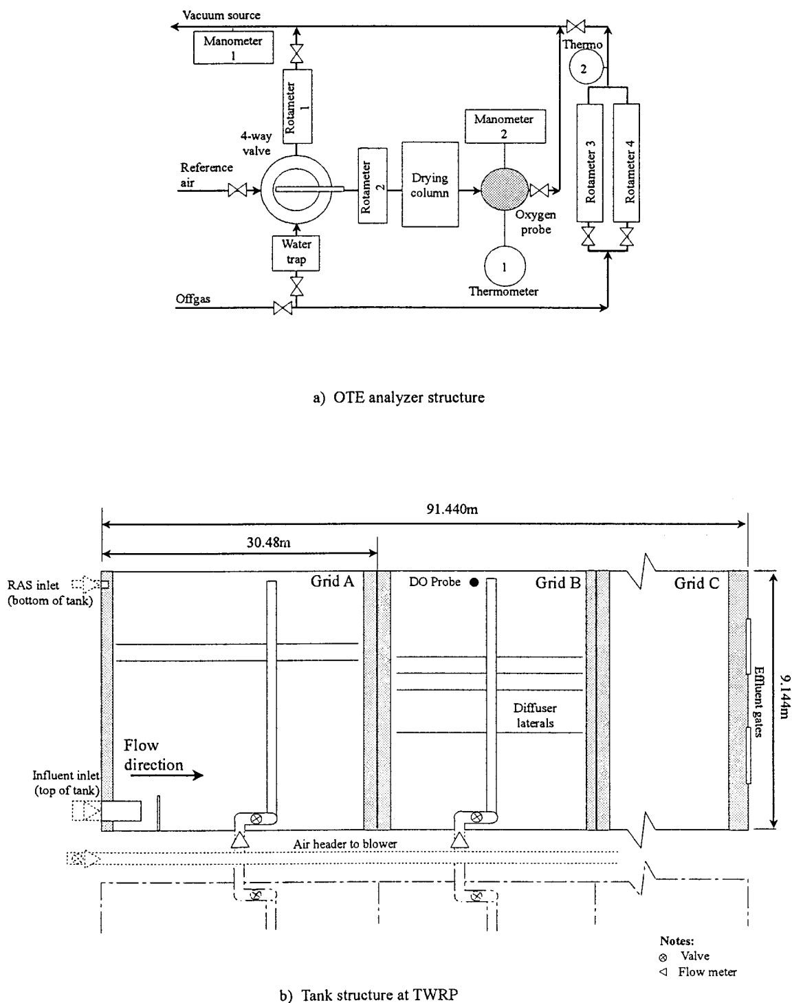
Figure 1—Plan views of (a) analyzer structure and (b) basin design.
