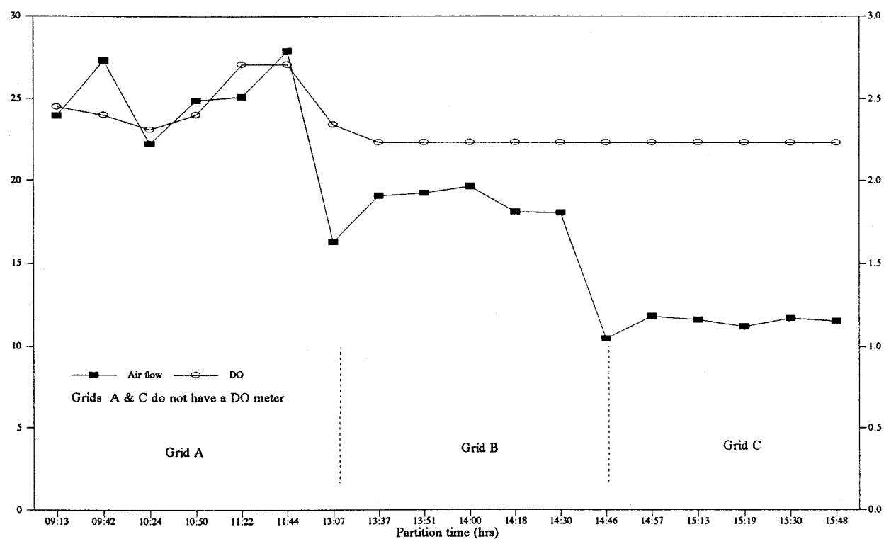
(a) Air flow rate and DO
