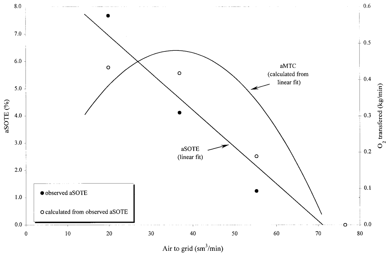
Figure 3—Efficiency and MTC for grid A, tank 15, TWRP, April 14, 1999.
