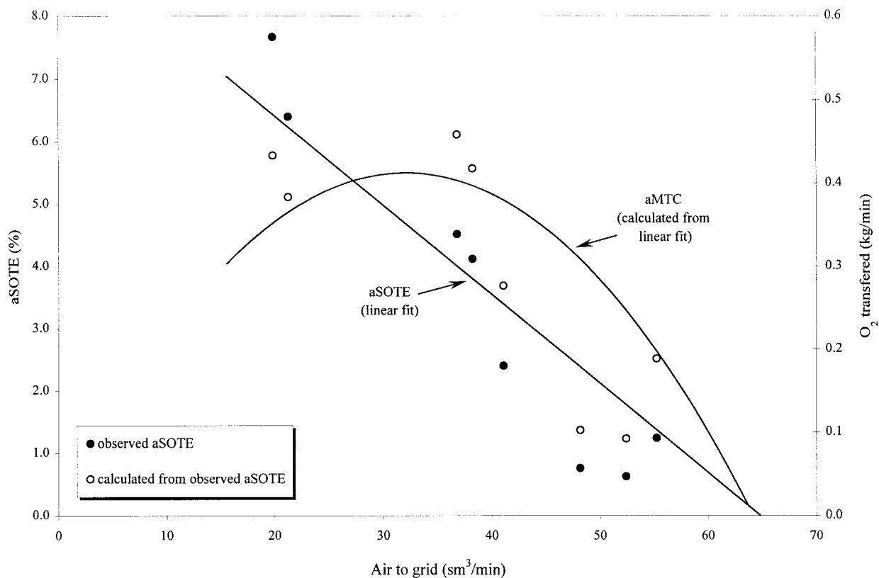
Figure 4—Efficiency and MTC for grid A, tank 15, TWRP, April 13 and 14, 1999.
