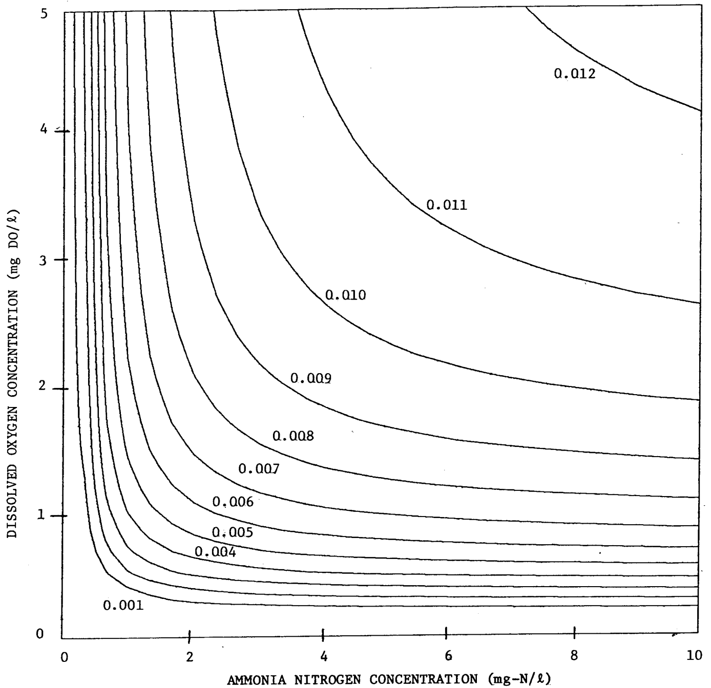
Figure 4: Net Growth Rate Contours Versus Ammonia Nitrogen and Dissolved Oxygen Concentration. (Numbers on curves indicate growth rate, \text{hrs}^{-1} . (After Stenstrom and Poduska, 1980))
