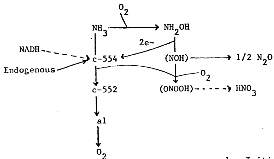
1a: Initial State of Ammonia Oxidation
