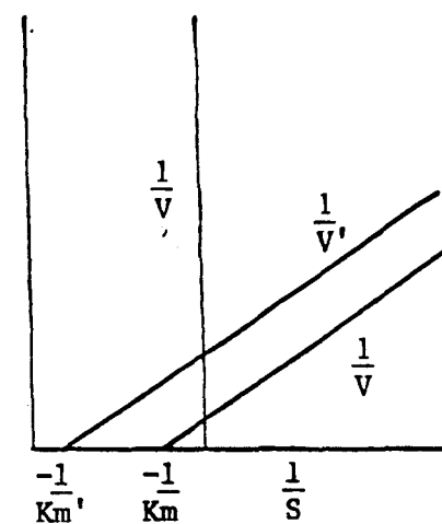
Figure 6: Effect of Inhibitors on Various Types on Lineweaver-Burke Plots of Substrate Concentration on Enzyme Reaction Velocity. V' and K_m' equal to V and K_m in the presence of an inhibitor.
