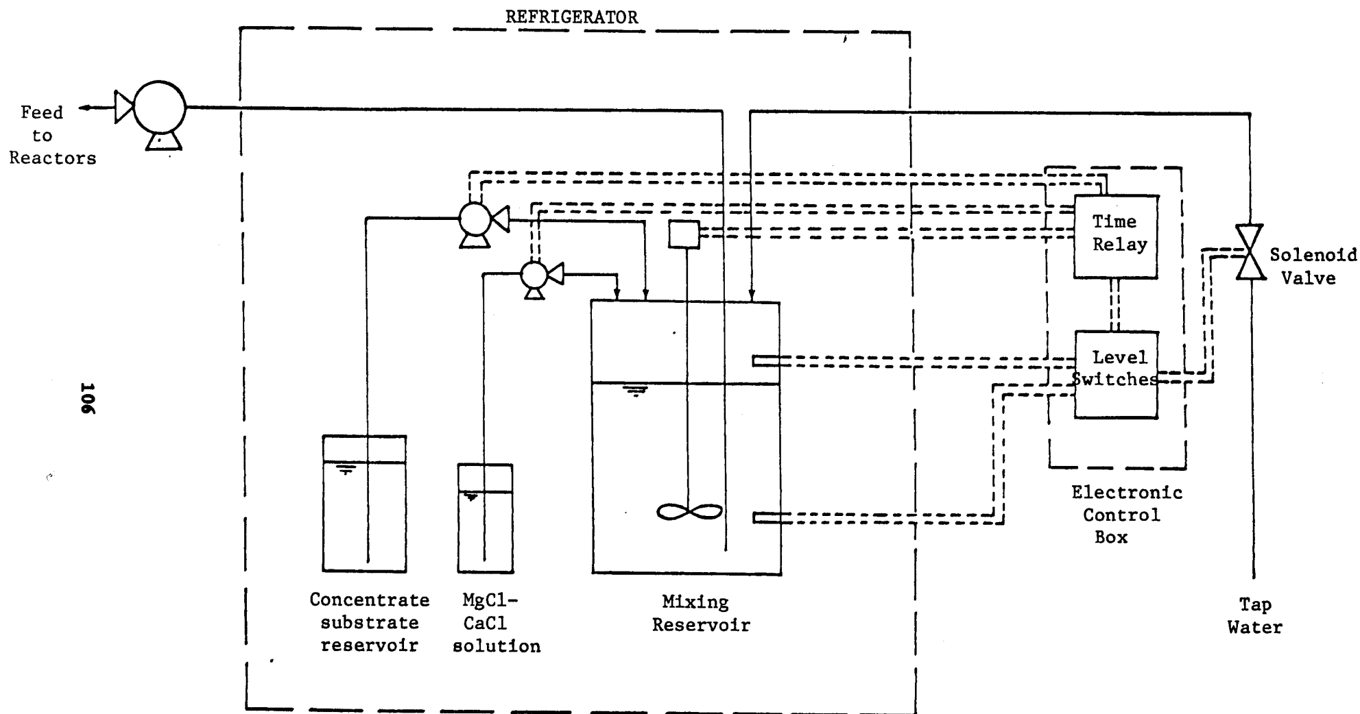
Figure 8: Schematic of Substrate Dilution System
