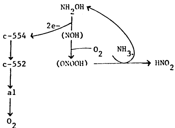
1b: Steady State
