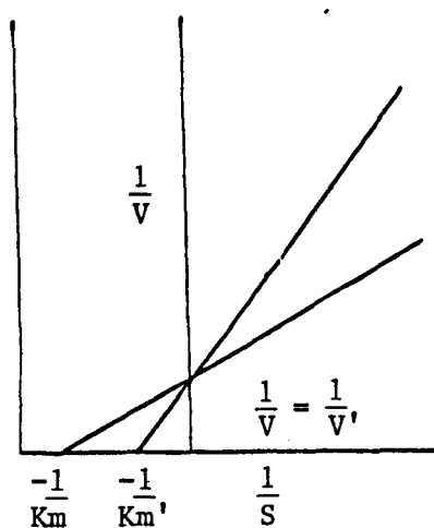
Figure 6: Effect of Inhibitors on Various Types on Lineweaver-Burke Plots of Substrate Concentration on Enzyme Reaction Velocity. V' and K_m' equal to V and K_m in the presence of an inhibitor.
