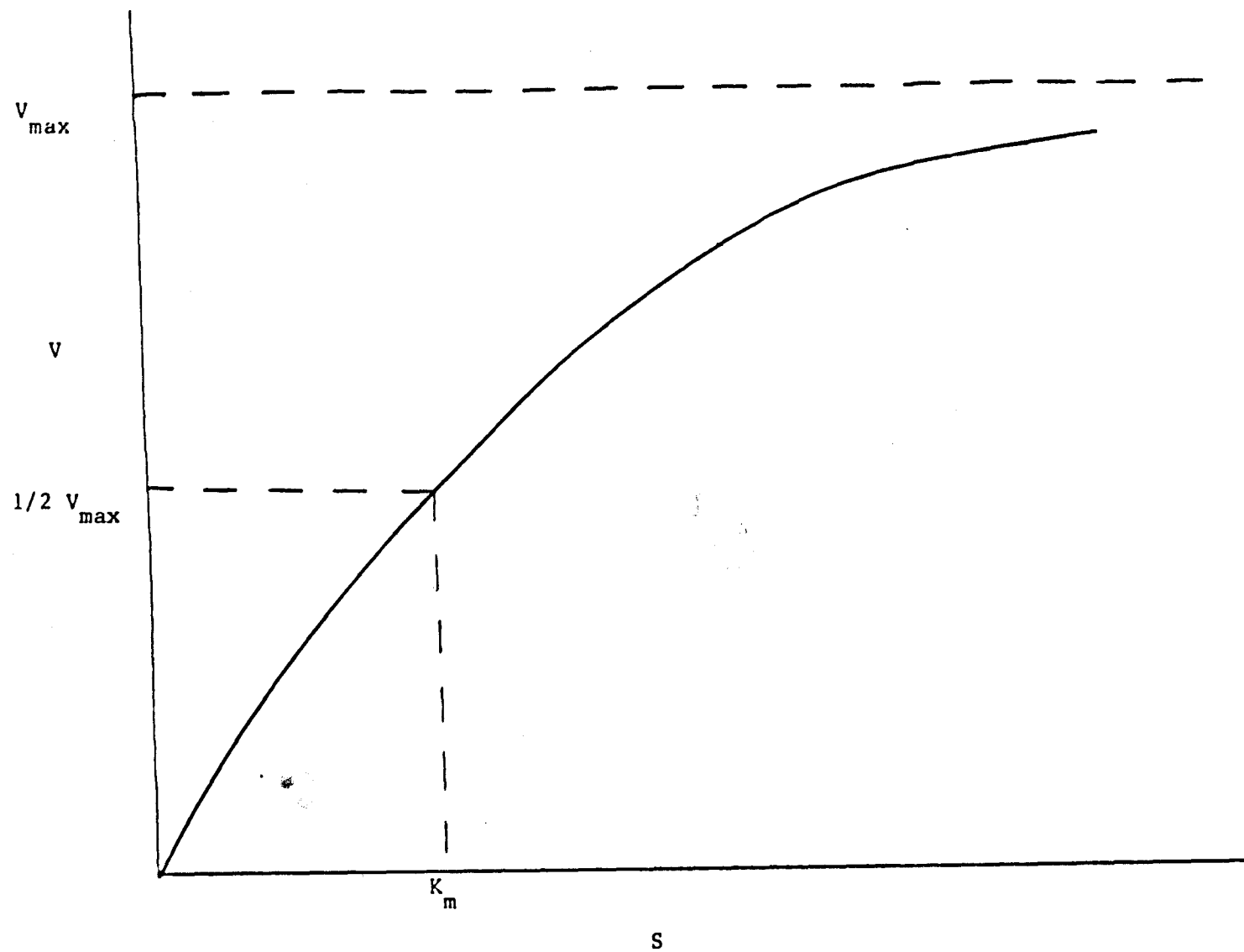
Figure 5: Plot of the Michealis-Menten Equation
