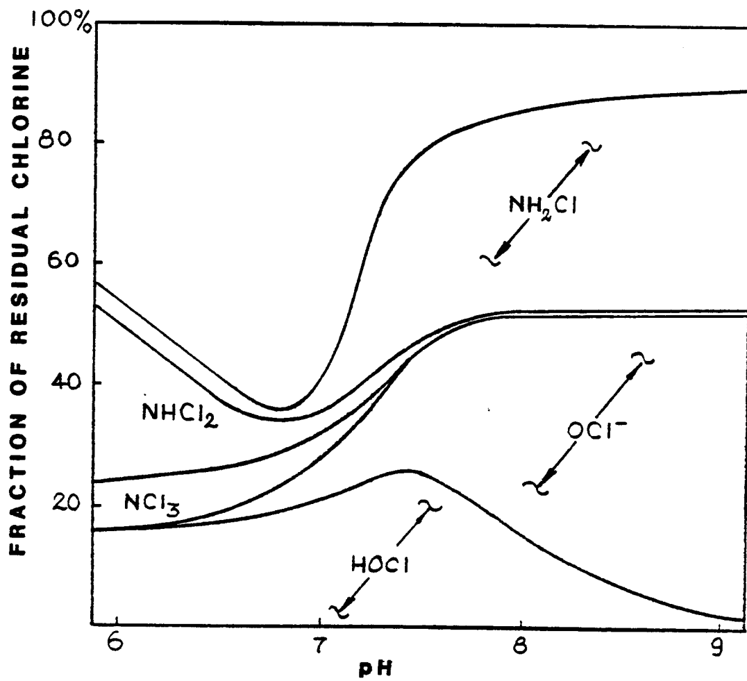
Figure 2-3: Variation of Chlorine Residual with pH after 10 Minute Contact Time for Cl/N Ratio of 2.37
