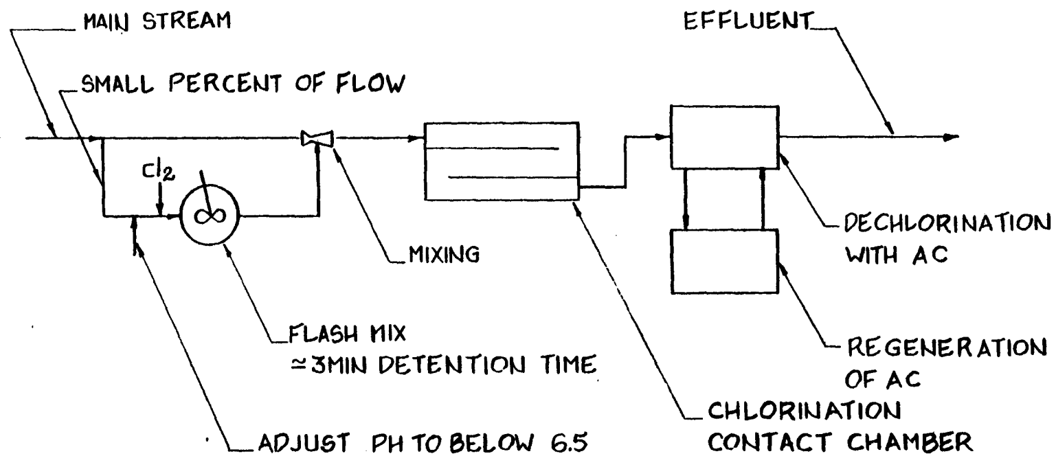
Figure 6-13: Proposed Dichloramine Disinfection Process
