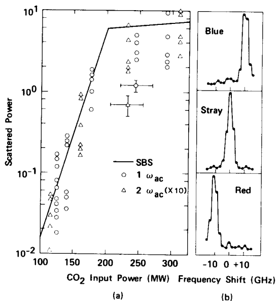
FIG. 1. (a) Thomson-scattered power at the fundamental (circles) and second harmonic (triangles) of the SBS ion wave vs pump power. The solid line summarizes previous data on SBS reflectivity. (b) Spectra of Thomson-scattered ruby light when k -matched to +2k_0 (red shift) and -2k_0 (blue shift). The "stray" curve shows the instrument width.
