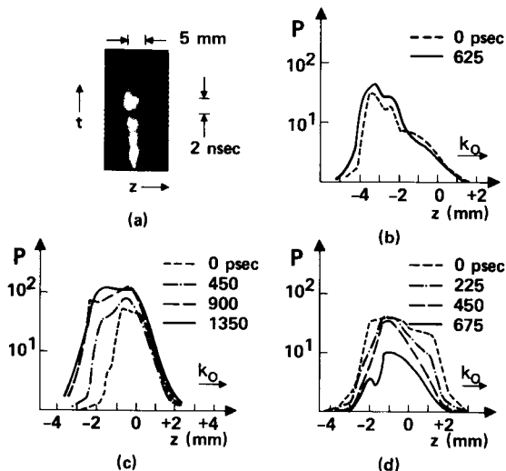
FIG. 2. (a) Typical streak image at 15-nsec full frame. (b)–(d) Microdensitometer scans of streak images of three shots showing relative scattered power P \propto (\bar{n}/n_0)^2 vs z at various times during the pulse. One acoustic period is \approx 100 psec. The CO 2 best focus is at z = 0 .
