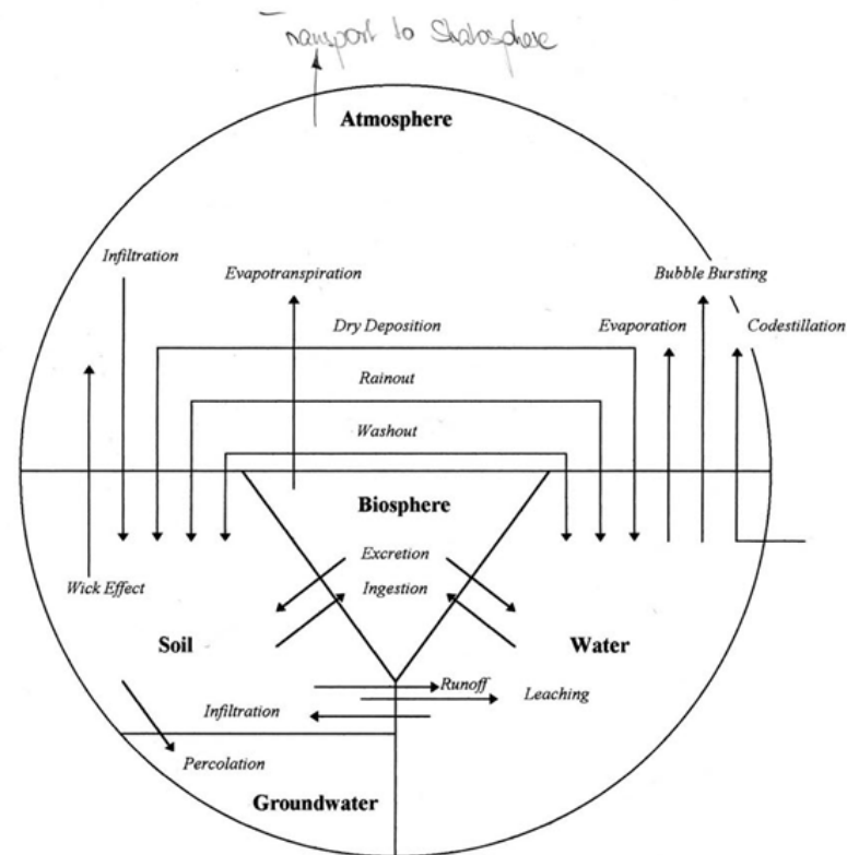
The famous 'Whitman Model' - transport mechanisms between environmental compartments
