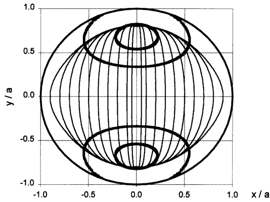
Figure 4. Electric field pattern corresponding to the mode shown in figure 1. The broad lines are contours of constant energy deposition (at 90% and 50% of maximum) for the plane-polarized component.
