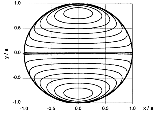
Figure 1. Pattern of magnetic field lines for the plane-polarized component of a helicon wave comprising superposed m = +1 and m = -1 azimuthal modes. Assumed parameters: 800 G, 10^{13} cm ^{-3} , 13.56 MHz, 5 cm radius. This pattern is fixed with respect to the antenna.
