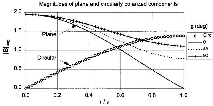
Figure 3. Relative time-averaged amplitudes of the plane and circularly polarized components.
