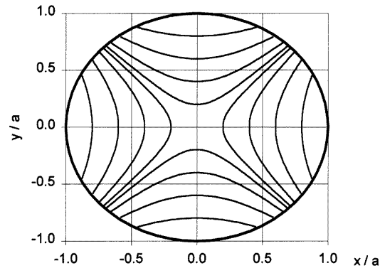
Figure 6. Electric field pattern for a plane-polarized m = 2 wave.
