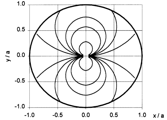
Figure 2. Same as figure 1, but for the circularly polarized component. This pattern rotates in the clockwise direction if B_\theta is out of the plane of the page. The B_z component of the field is not shown, and the line spacing is not indicative of the field strength.
