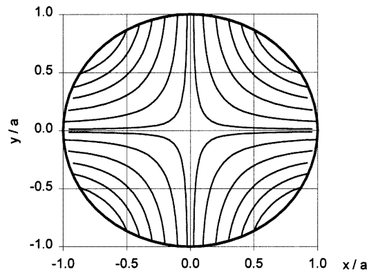
Figure 5. Magnetic field pattern for a plane-polarized m = 2 wave.
